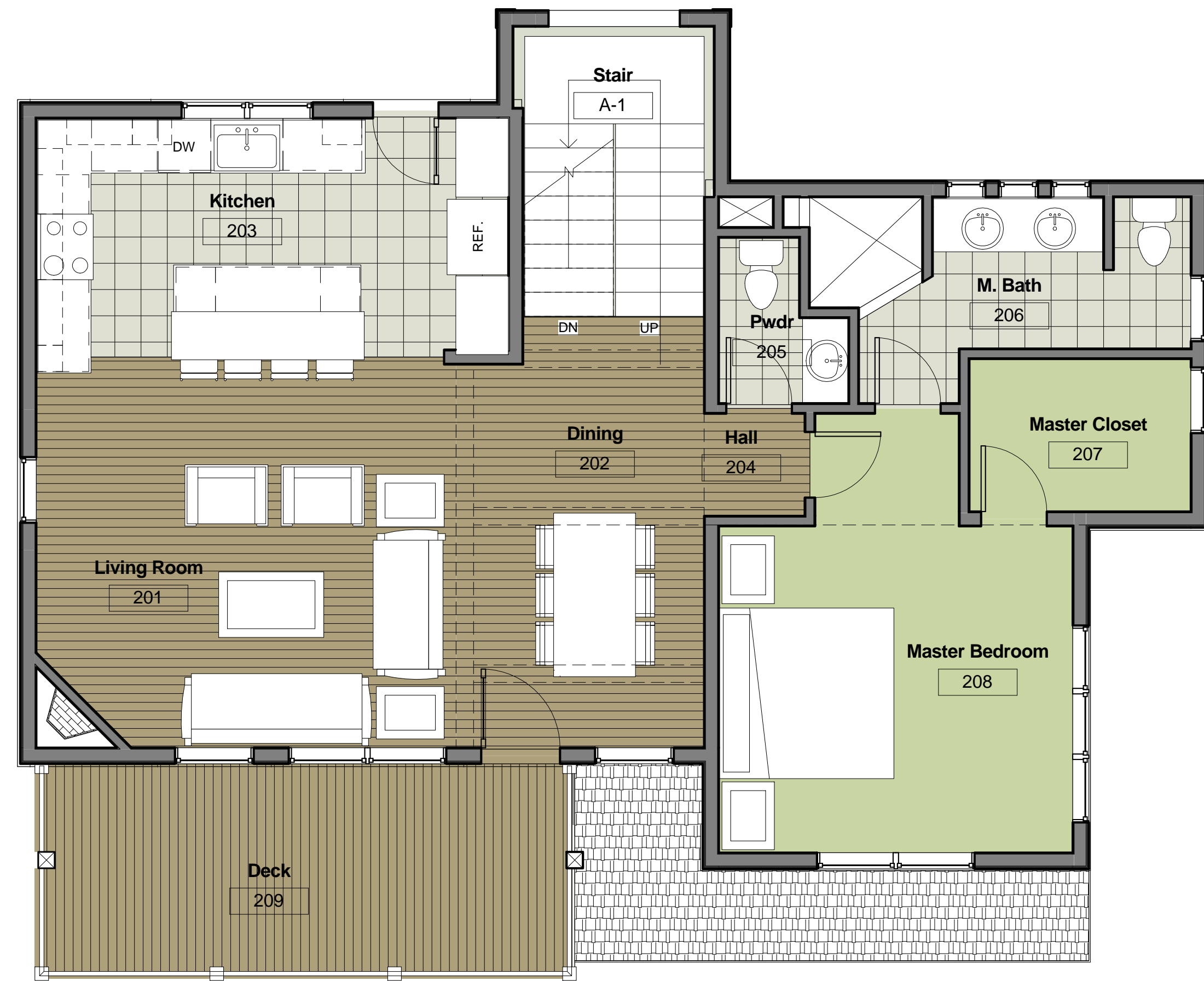
2 Main Floor- 1/4" = 1'-0"
