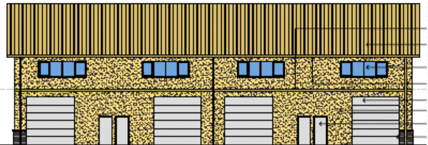
2 SOUTH ELEVATION 1/2" = 10'-0"
